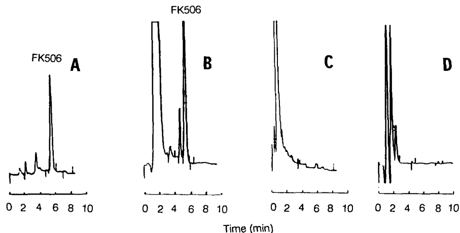
FIG. 2. Chromatograms of FK 506 solutions; (A) pure FK 506 solution in methanol ( 5 \mu\text{g mL}^{-1} ); (B) FK 506 solution in simulated gastric fluid ( 25 \mu\text{g mL}^{-1} ); (C) FK 506 solution degraded by acid and heat and (D) FK 506 degraded at pH 10.
